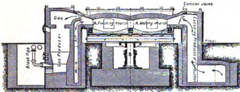
Fig. 96. Diagrammatic Section of the Pietzka Puddling Furnace.
